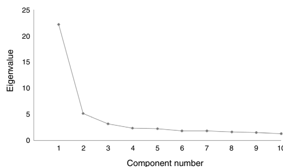
Figure 1. Scree plot of eigenvalues after exploratory factor analysis.
